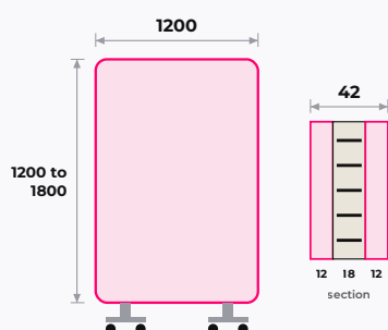
Screen 1200 wide, shown on castors, with a section through the board. Not to scale.
